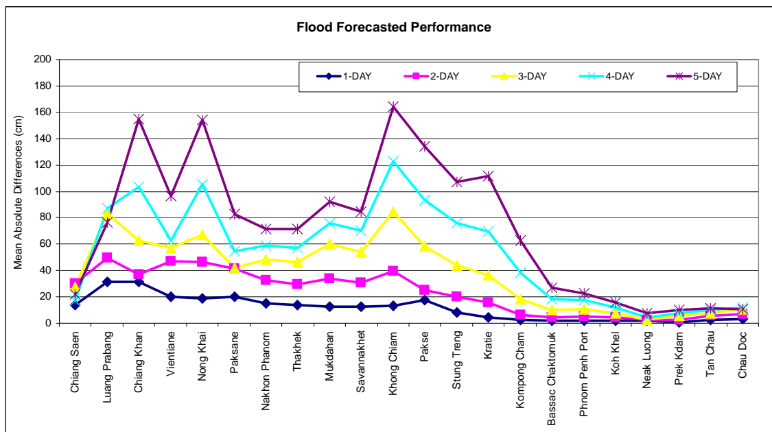
Figure B1: Average flood forecast accuracy along the Mekong mainstream (from 07 th – 14 th August 2017)
